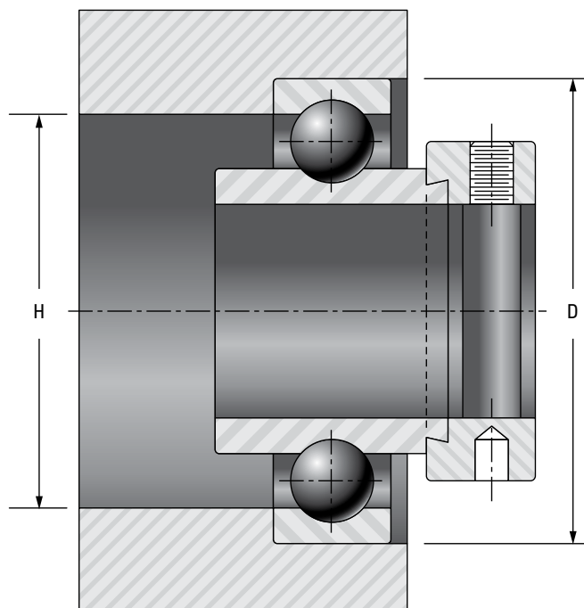
Fig. 35. Wide inner ring ball bearing.
