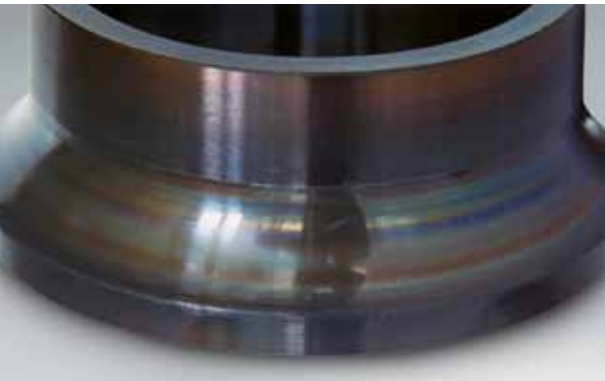
Photo 18.1 Part: Inner ring of an angular contact ball bearing Symptom: Bluish or purplish discoloration on raceway surface Cause: Heat generation due to poor lubrication
